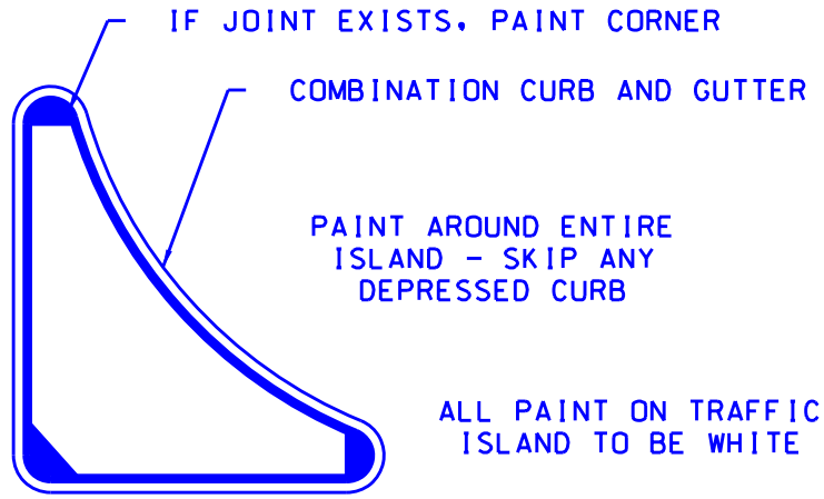
TYPICAL PAVEMENT MARKINGS AT ISLAND
