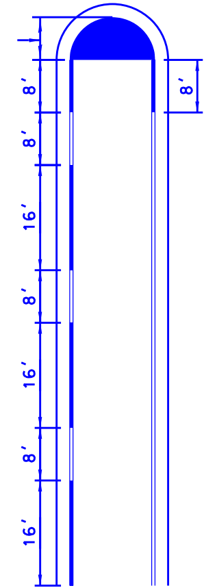
TYPICAL PAVEMENT MARKINGS AT MEDIAN NOSE
