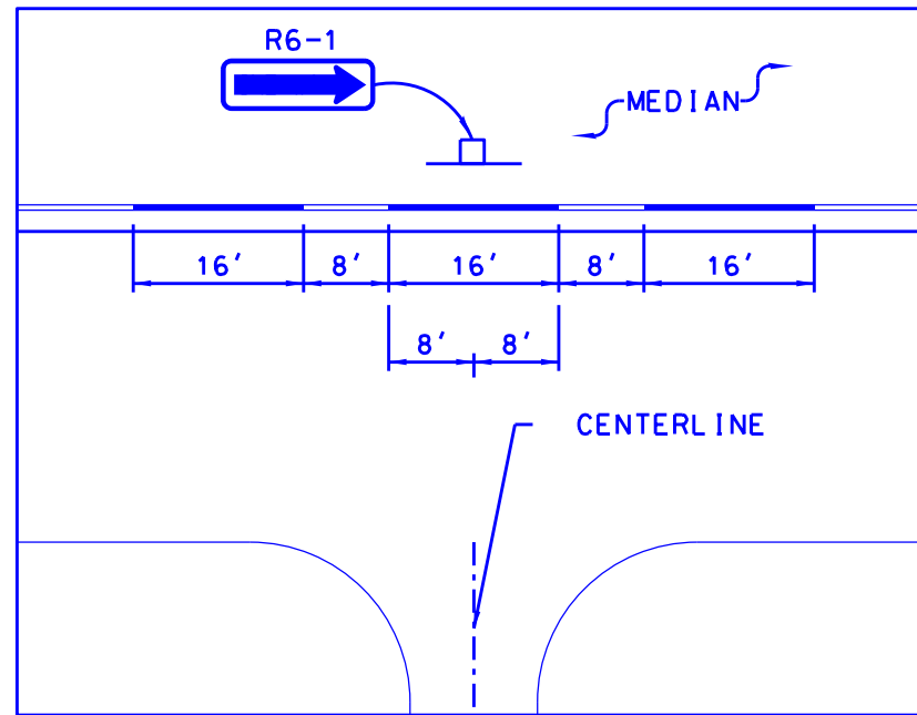
SKIPS AT DRIVEWAYS OR SIDE STREETS
